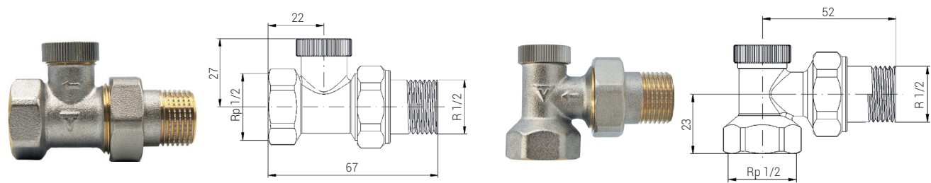
FP / FK control valve, straight or angular version. F 1/2" x M 1/2".
