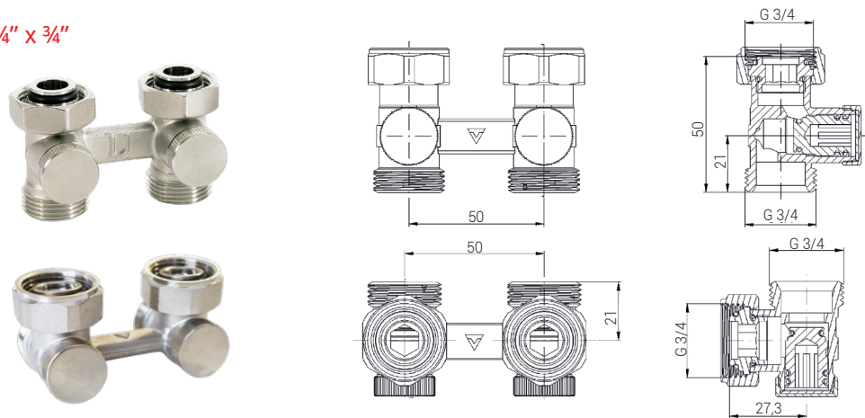
V TYPE double-pipe connection valve, F 3/4" x M 3/4". Straight or angular version. Connection spacing 50 mm.
