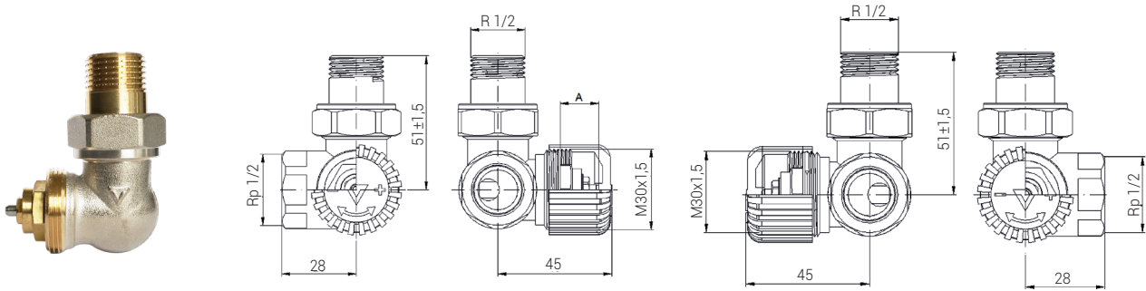
ARCUS thermostatic valve, axial, left or right version. F 1/2" x M 1/2". Thermostatic head mounting thread M30x1,5. Economy version. Without pre-setting.
