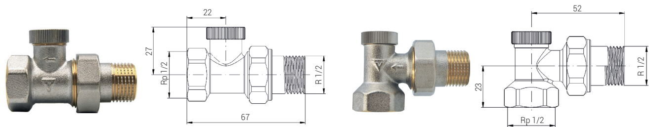
FP / FK control valve, straight or angular version. F 1/2" x M 1/2".
