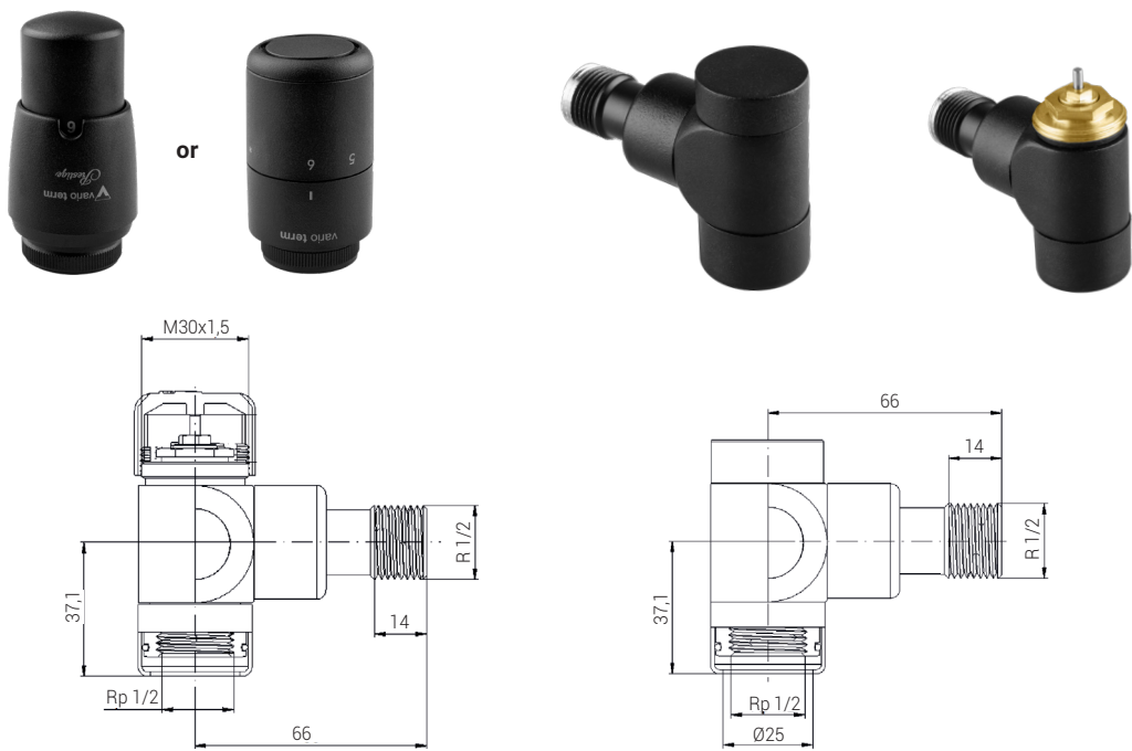
LUX II thermostatic set. Angular version, F ½" x M ½".
