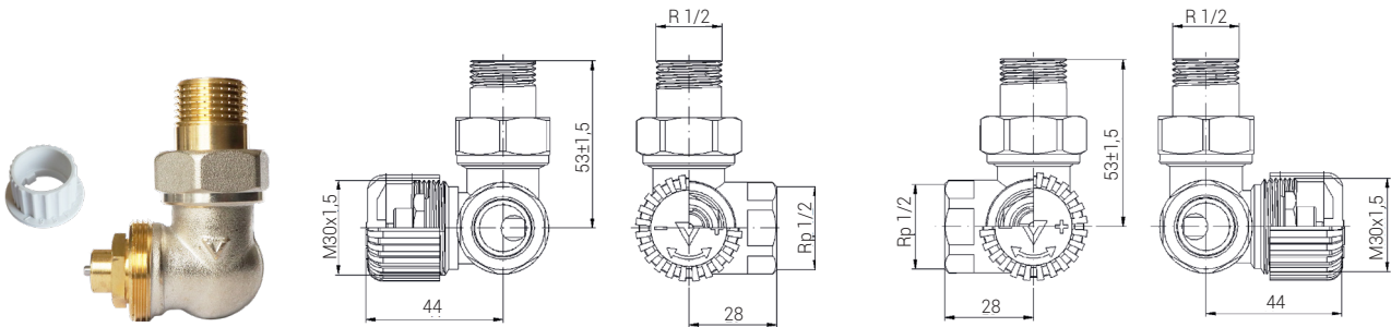
MASTER thermostatic valve, axial, left or right version. F 1/2" x M 1/2". Thermostatic head mounting thread M30x1,5. Economy version. Pre-setting. KN-01 setting key included. PEX version has a short PEX connector (16x2).
