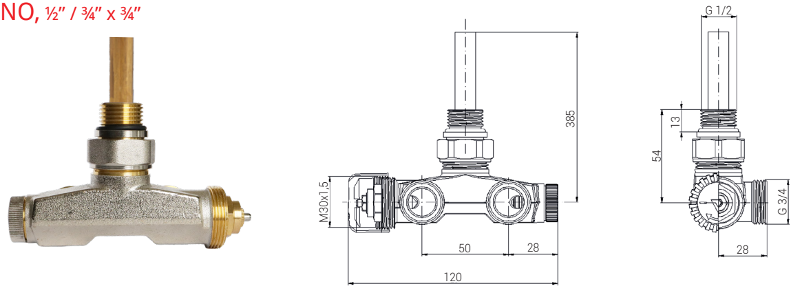
UNO connection, right version, with immersion tube. M 1/2" x M 3/4". Connection spacing for 50 mm installation. Thermostatic head mounting thread M30x1,5. Economy version. The setting is regulated by a return valve.
