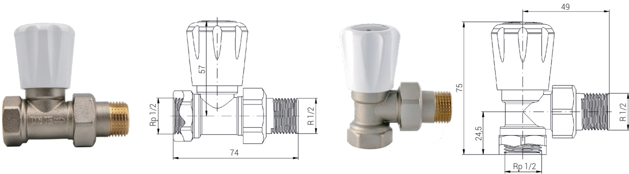
SWING II control valve, straight or angular version. F 1/2" x M 1/2". Large flow diameter. Control knob protected by a plastic cover.
